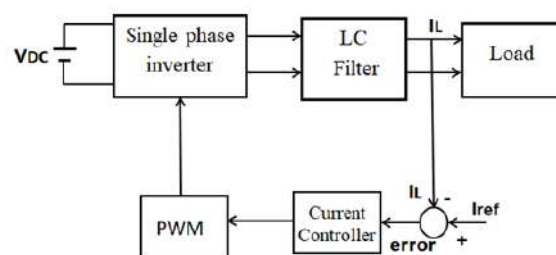
Fig.1 Closed loop Block diagram of single-phase inverter
